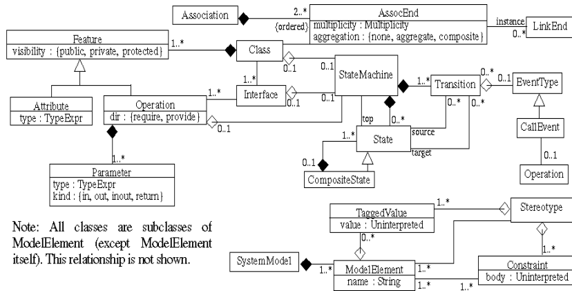
Figure 1. Simplified UML meta-model (adapted from [21]).
